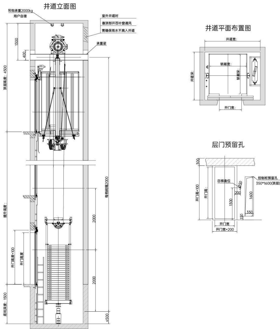
标准规格及尺寸 (高速梯参数另算) STANDARD SPECIFICATIONS AND DIMENSIONS
