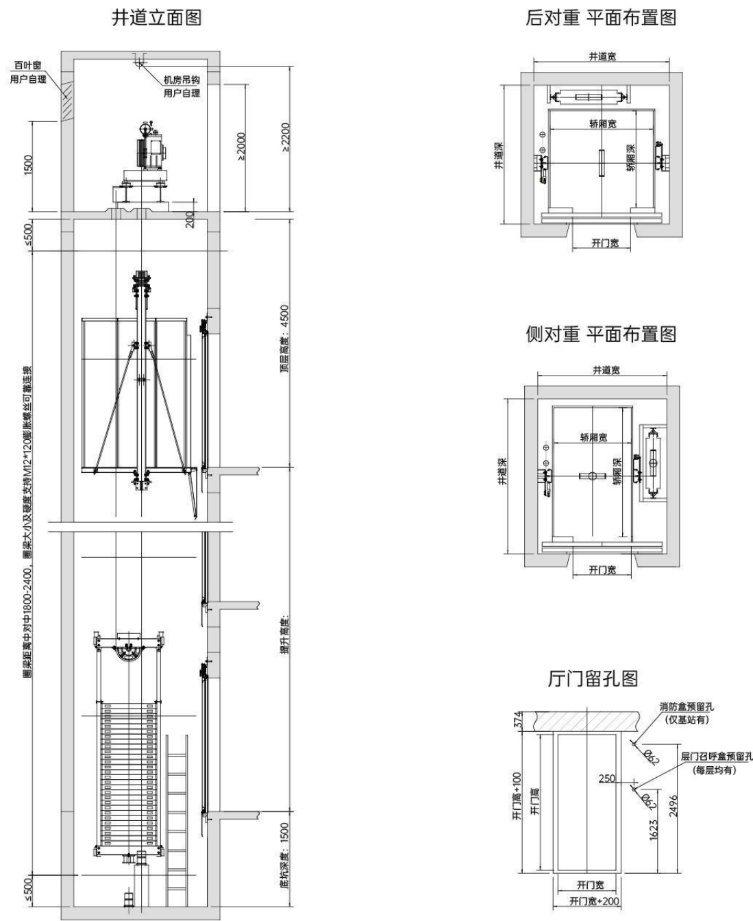
标准规格及尺寸 (高速梯参数另算) STANDARD SPECIFICATIONS AND DIMENSIONS
